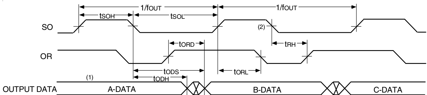
Figure 5. Output Timing
