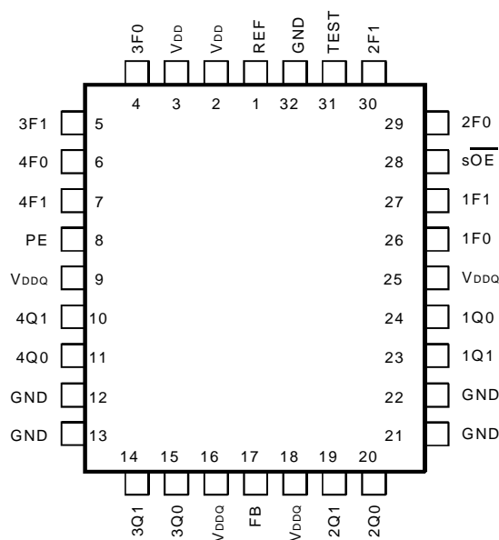
PLCC TOP VIEW
