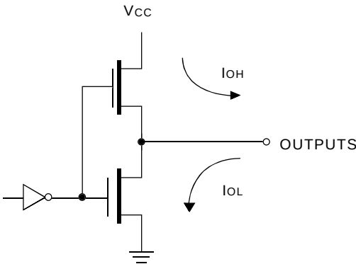
Output Interface Circuit
