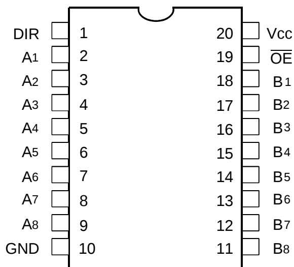
QSOP/ SOIC/ SSOP/ TSSOP TOP VIEW
