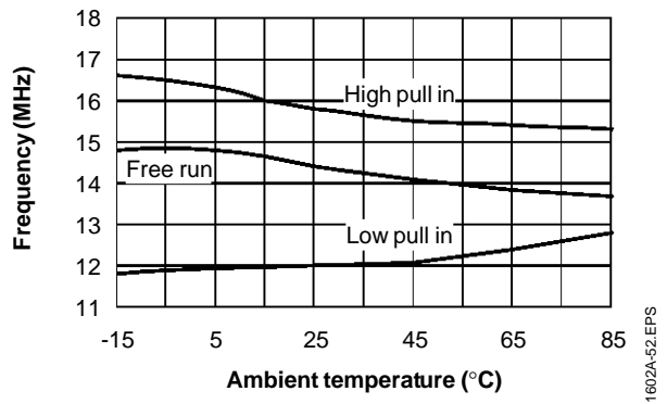
Figure 34 : Pull-in Range and Free Run Frequency (143Mb/s)
