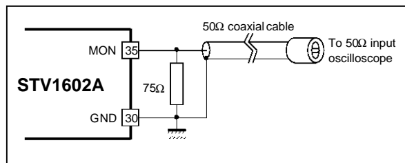
Figure 14 : Equalized Waveforms Monitoring
