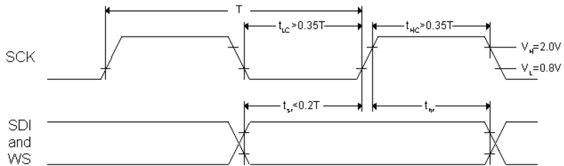
Timing For I 2 S Receiver
