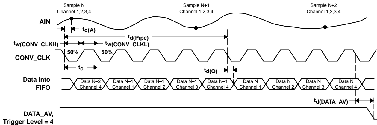
Figure 5. Timing of Continuous Conversion Mode (4-channel operation)
