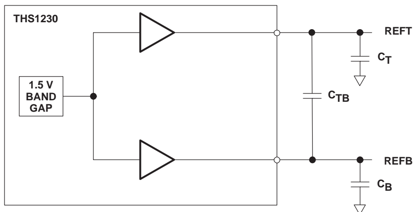
Figure 1. Reference Generation
