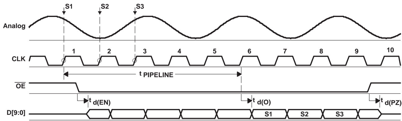
Figure 2. Input Timing
