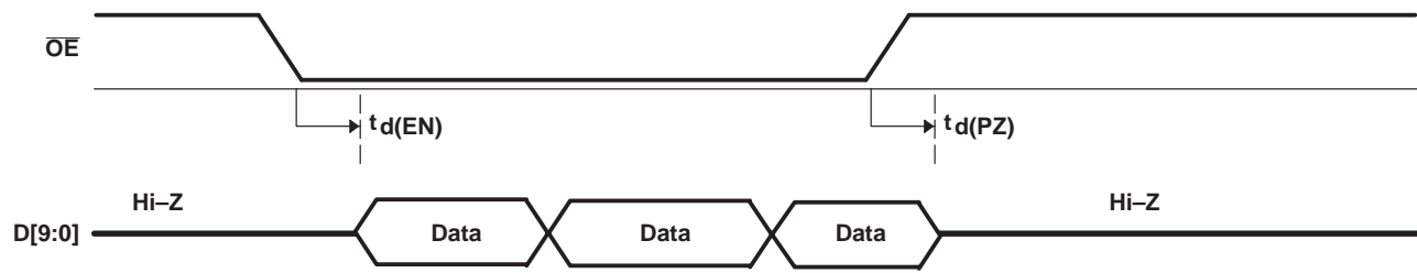
Figure 3. Output Timing
