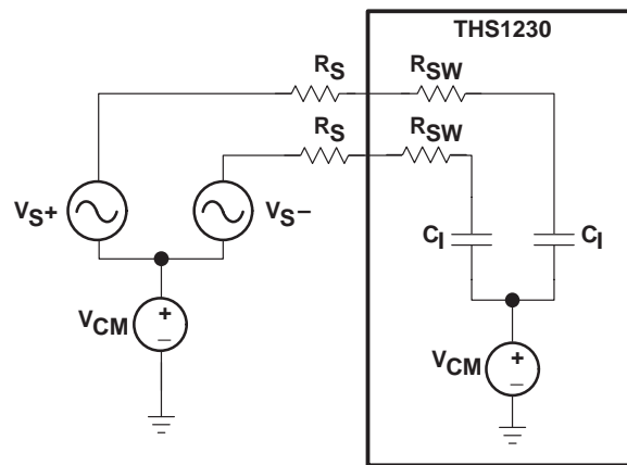
Figure 15. Simplified Equivalent Input Circuit
