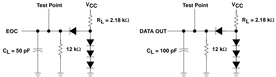
Figure 2. Load Circuits
