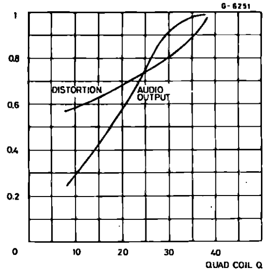
Figure 6 : Effect of Quadrature Coil "Q" on Audio Level and Distortion
