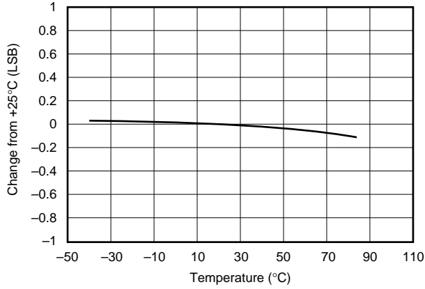
CHANGE IN BIPOLAR OFFSET vs TEMPERATURE
