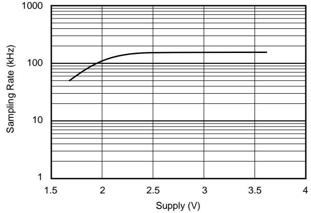
MAXIMUM SAMPLING RATE vs SUPPLY VOLTAGE
