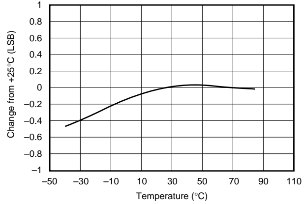
CHANGE IN GAIN vs TEMPERATURE
