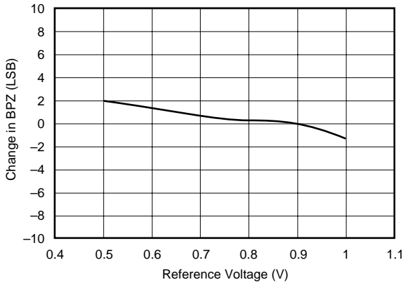
CHANGE IN BPZ vs REFERENCE VOLTAGE
