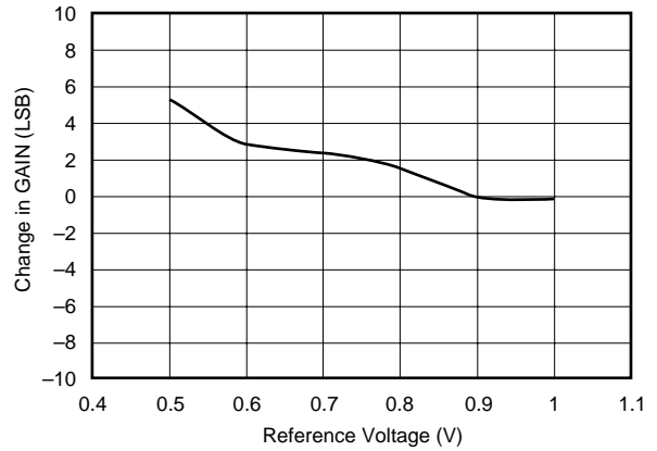
CHANGE IN GAIN vs REFERENCE VOLTAGE
