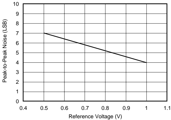
NOISE vs REFERENCE VOLTAGE
