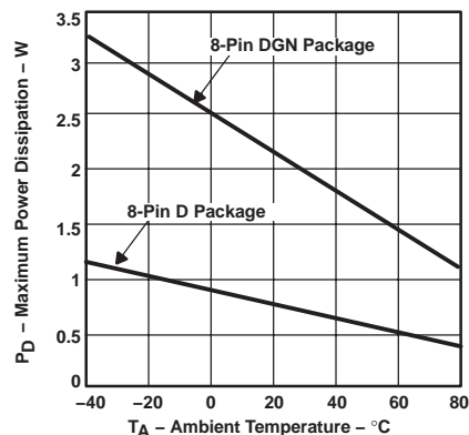
Figure 113. Maximum Power Dissipation vs Ambient Temperature
