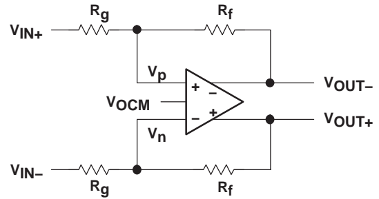
Diagram For Input Common-Mode Range Equations Figure 95
