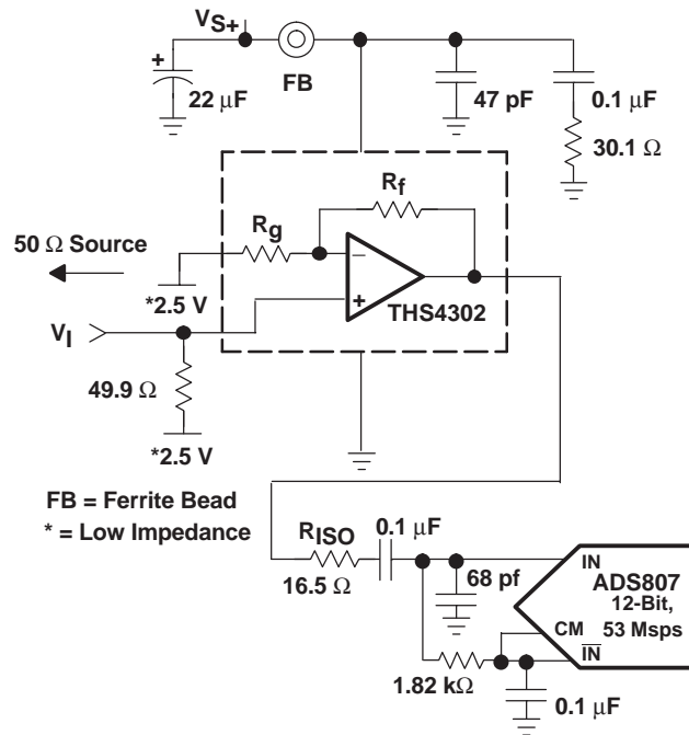
Figure 45. Driving an ADC With a Single-Ended Input
