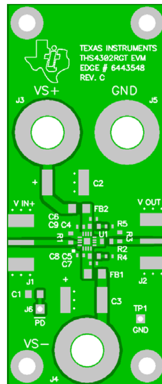
Figure 51. THS4302EVM Layout (Top Layer and Silkscreen Layer)
