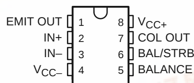
LM211 . . . D PACKAGE (TOP VIEW)
