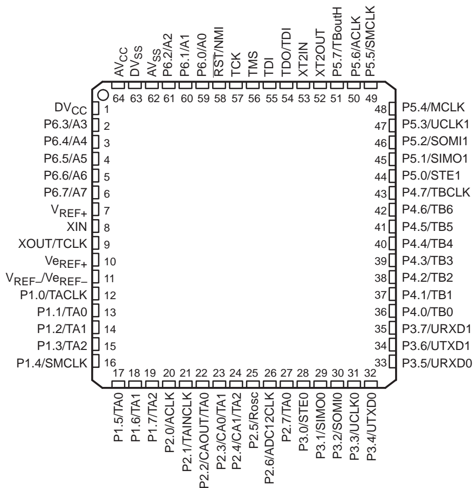
PM, PAG PACKAGE (TOP VIEW)
