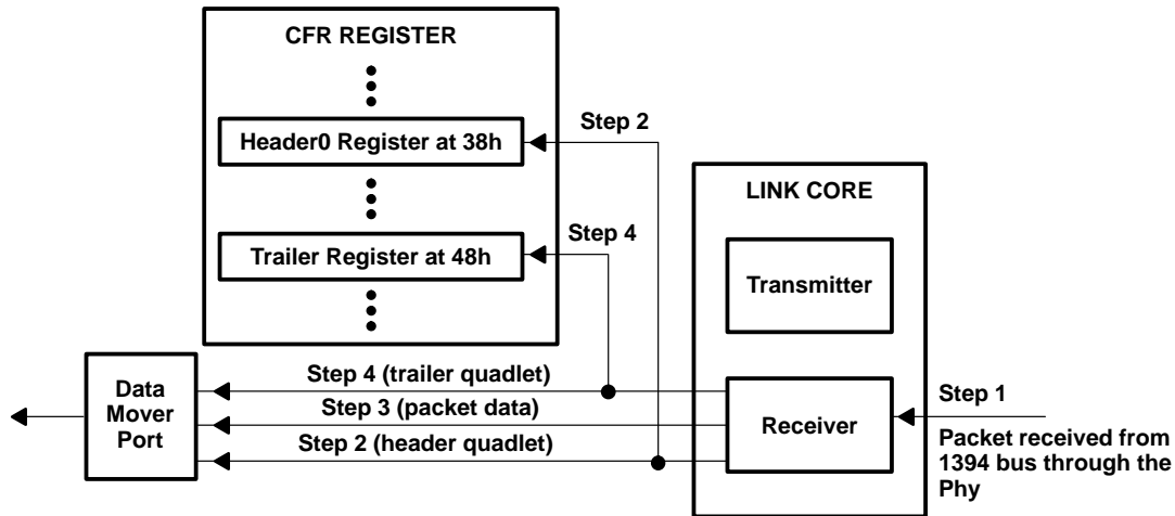
Figure 5-6. Isochronous Receive With Header and Trailer
