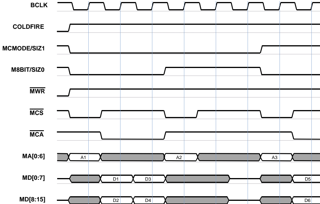
Figure 3–13. ColdFire Read
