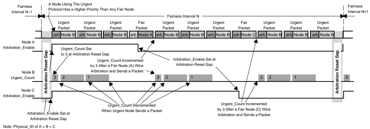
Figure 6–11. Urgent Arbitration
