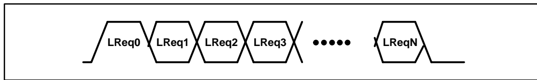
Figure 6-2. LREQ Timing
