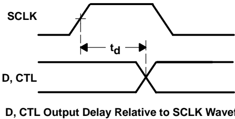
Figure 4–1. Parameter Measurement Information
