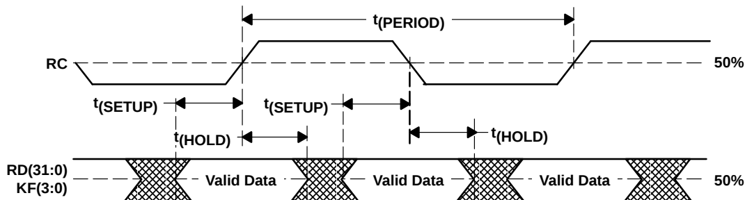
Figure 15. XGMII Receive Timing Diagram
