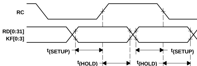
Figure 8. Receive Interface Timing
