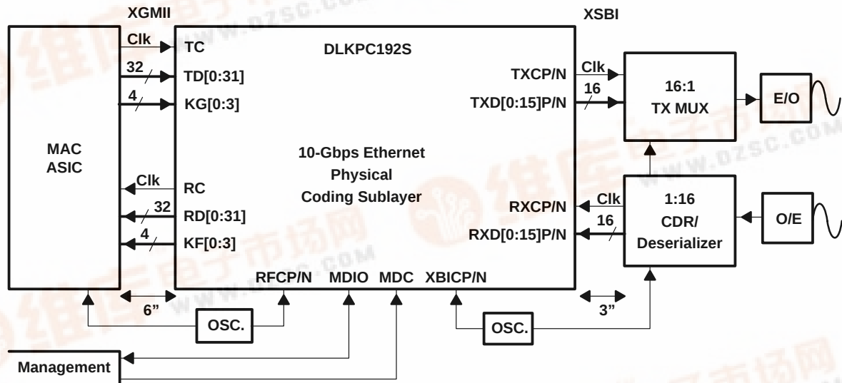
Figure 1. 10-Gbps Ethernet Short-PCB-Distance Implementation
