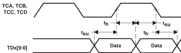
Figure 3–1. Transmit Interface Timing
