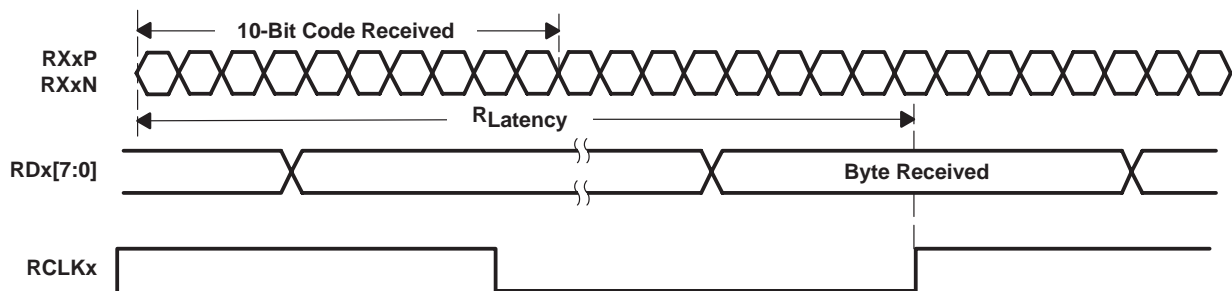
Figure 3–6. Receiver Latency
