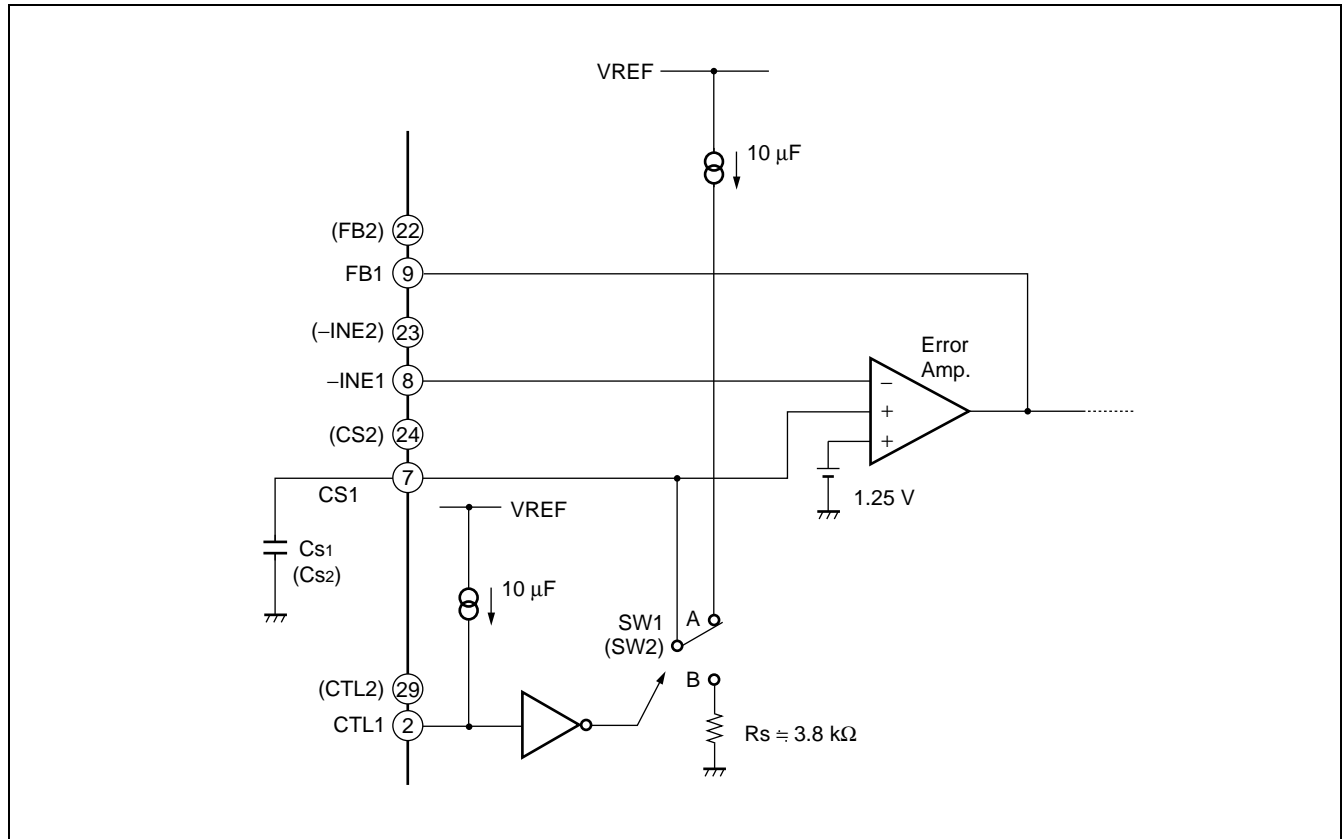
< Soft-start circuit >
