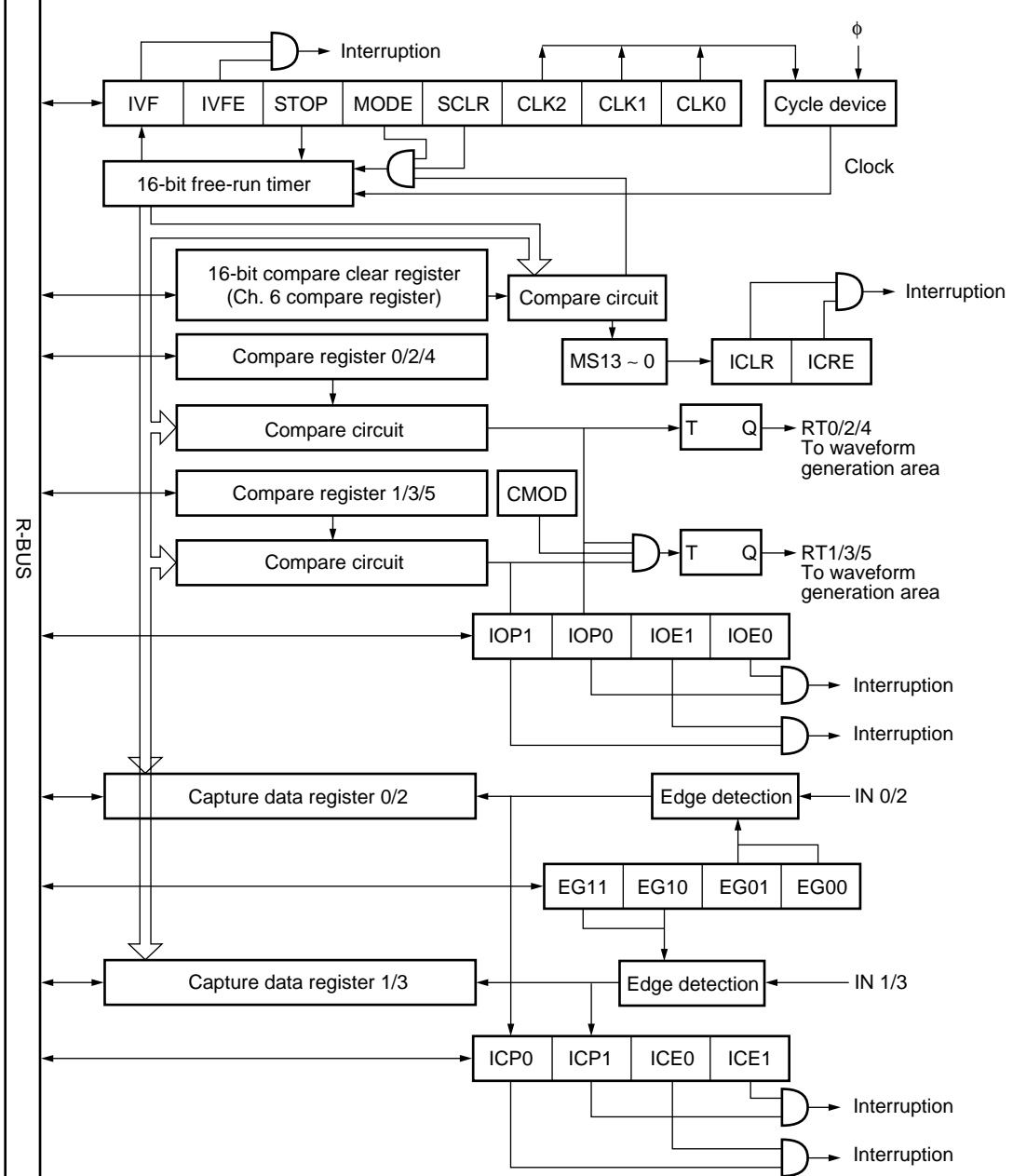
Block Diagram of PPG Timer for 1 Channel
