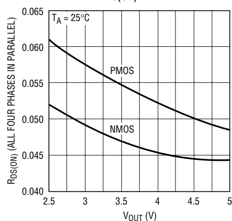
Effective R_{DS(ON)}
