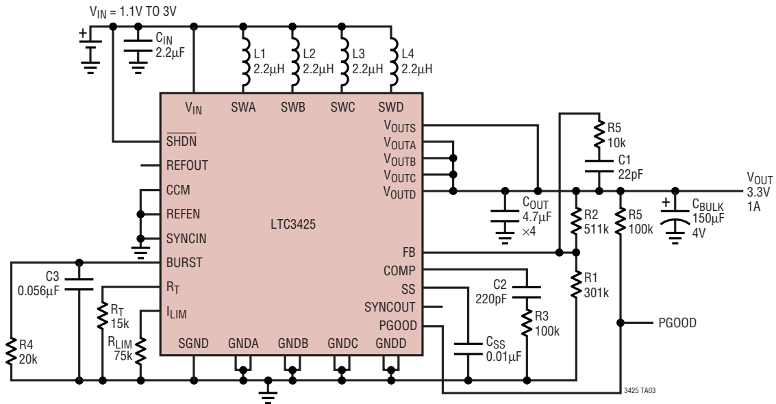
Single or Dual Cell to 3.3V Boost with Automatic Burst Mode Operation
