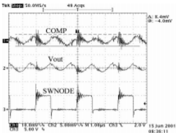
Figure 35. At Full- Load the Peak- to- Peak Voltage Ripple on the COMP Pin Should Be Less than 20 mV for a Well- Tuned/Stable Controller. Higher COMP Voltage Ripple Will Contribute to Output Voltage Jitter.
