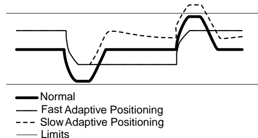
Figure 21. Adaptive Voltage Positioning
