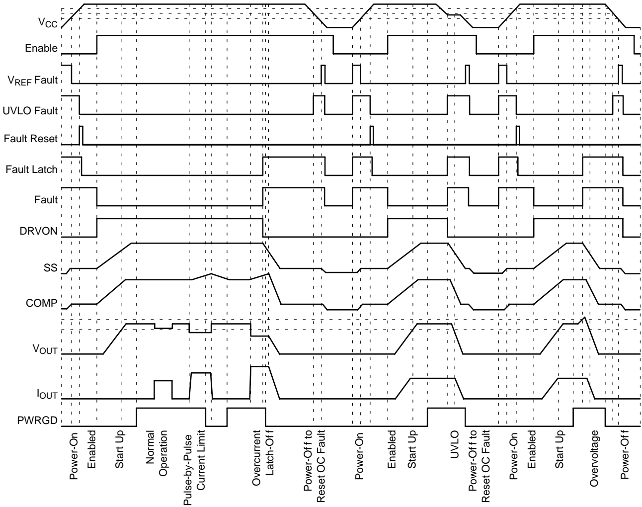
Figure 16. Operating Waveforms
