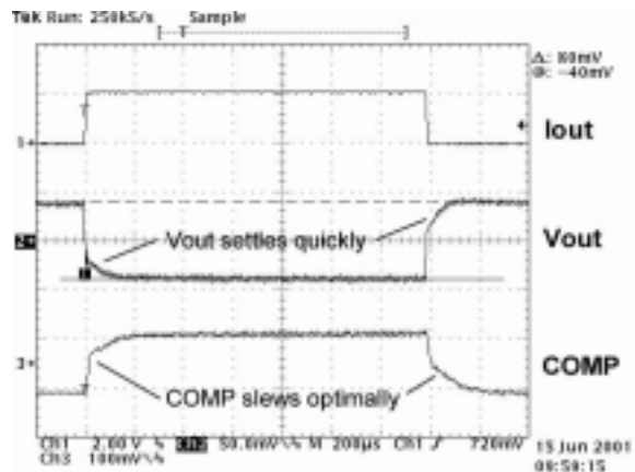
Figure 36. The Value of C_{AMP} Is Optimal. COMP Slews Quickly Without Spiking or Ringing. V_{OUT} Does Not Overshoot and Monotonically Settles to Its Final Value.
