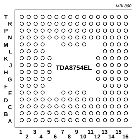
Fig.3 Pin configuration LBGA208 package.
