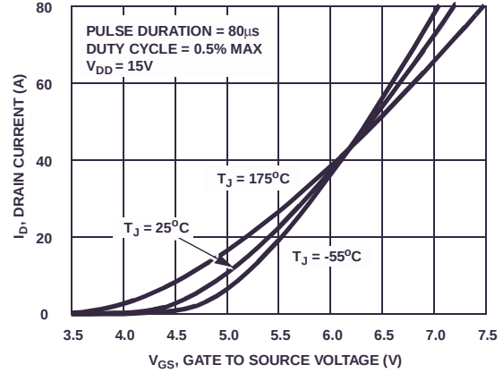
Figure 6. Transfer Characteristics
