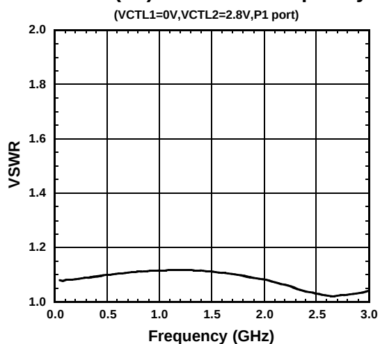
P1-P2(on) VSWR vs. Frequency
