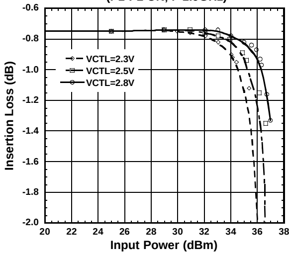
Insertion Loss vs. Input Power (P1-P2 ON, f=1.9\text{GHz} )
