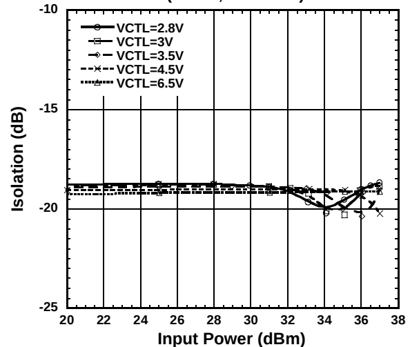
Isolation vs. Input Power (P1-P2, f=1.9\text{GHz} )
