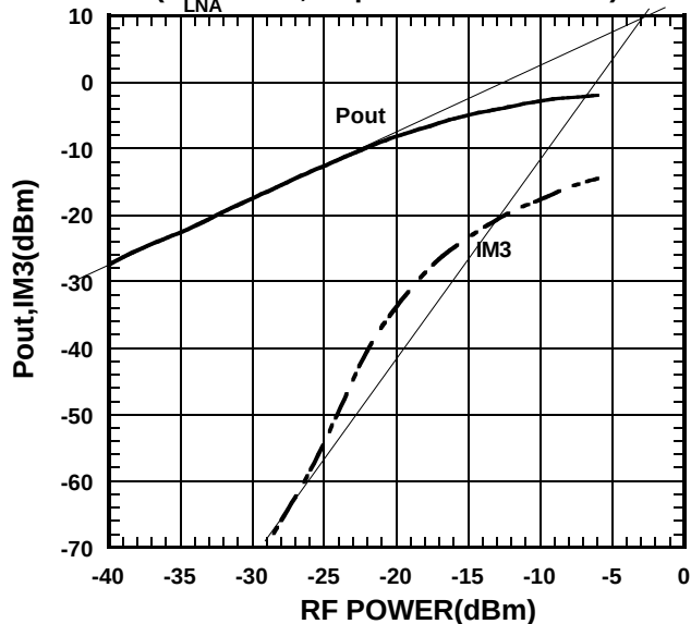
RF POWER vs. Pout, IM3
