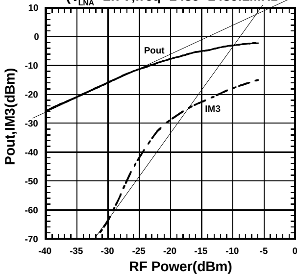
RF POWER vs. Pout,IM3 ( V_{LNA}=2.7\text{V} , freq=1489+1489.1MHz)
