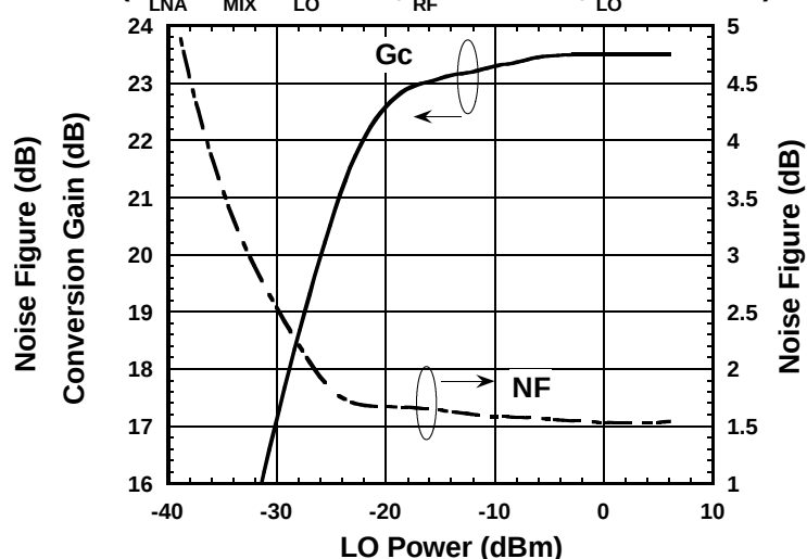
Conversion Gain , Noise Figure vs. LO Power
