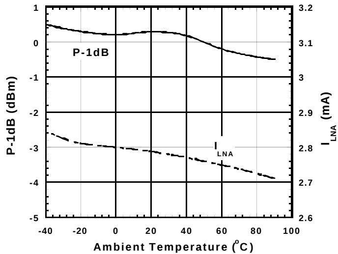
P-1dB, I_{\text{LNA}} vs. Temperature
