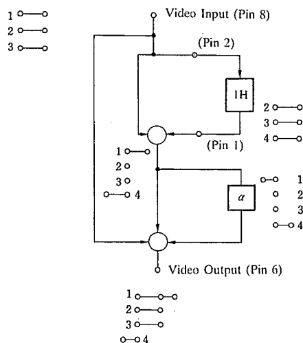
Fig.9 Block Explanation
