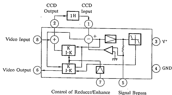
Fig.2 Block Diagram
