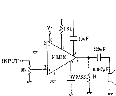
Amplifier 2
