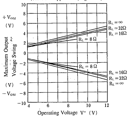
Maximum Output Voltage Swing vs. Operating Voltage (Standard Application, T_a = 25^\circ\text{C} )
