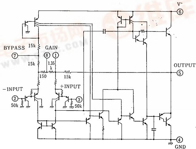
NJM386L
