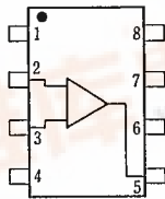
NJM386D NJM386M
