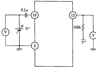
Test Circuit 3
