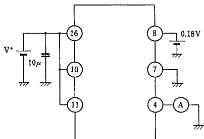
Test Circuit 13
