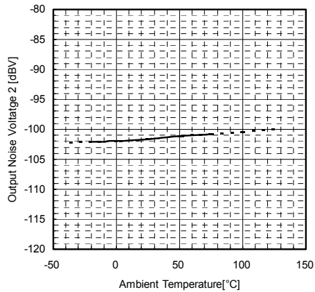
Output Noise Voltage 2 vs. Ambient Temperature V_{+}=9V , R_L=100\Omega , R_g=0\Omega , A-Weighted, MUTE=H
