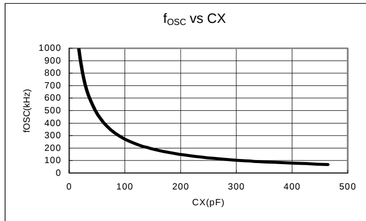
Figure 7 f_{OSC} vs. CX (Reference but not guaranteed)
