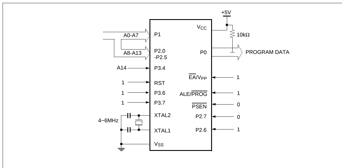
Figure 14. Program Verification
