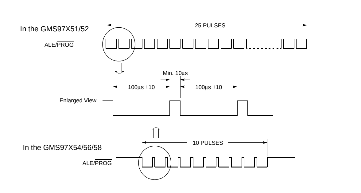
Figure 13. PROG Waveform
