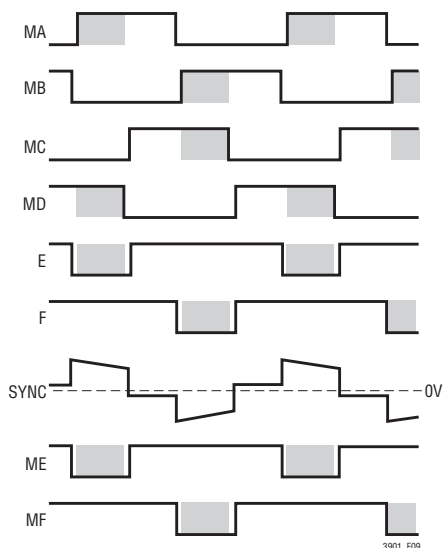
Figure 10. Full-Bridge Converter Switching Waveforms
