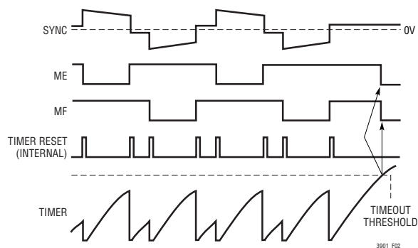
Figure 4. Timer Waveforms
