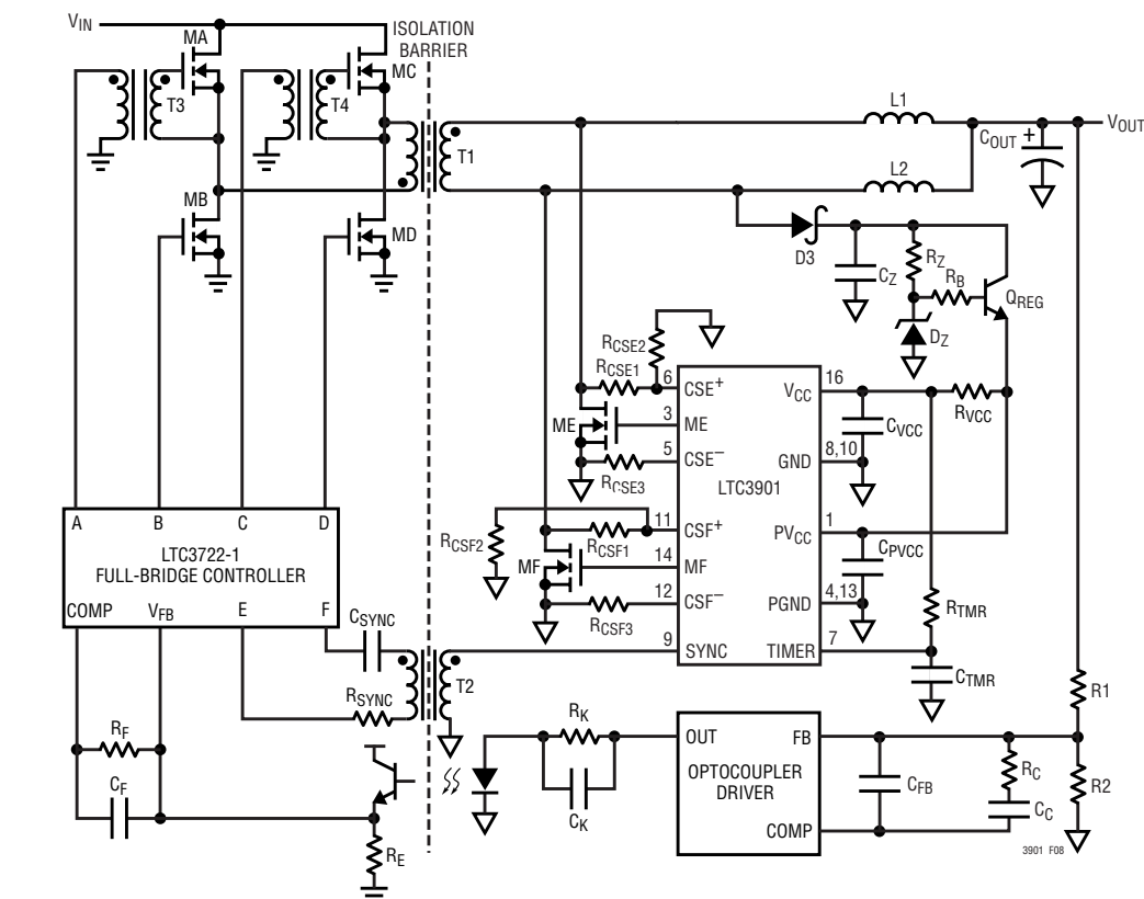
Figure 9. Simplified Isolated Full-Bridge Converter
