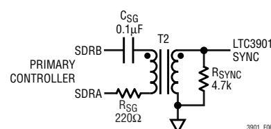
Figure 7. SYNC Input Circuit
