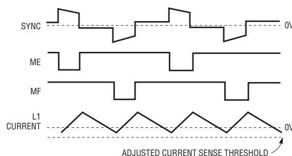
Figure 6b. Continuous Mode Operation with Adjusted Current Sense Threshold
