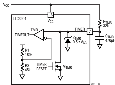
Figure 3. Timer Circuit
