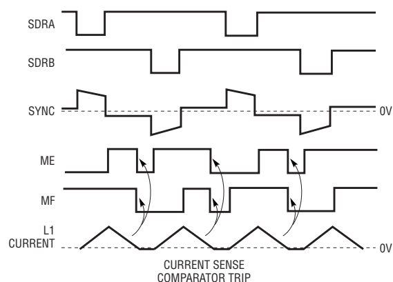
Figure 6a. Discontinuous Mode Operation at No Load
