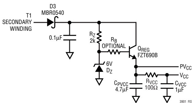
Figure 8. V_{CC}/PV_{CC} Regulator
