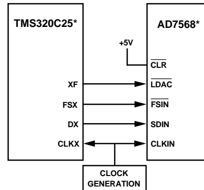
Figure 23. AD7568 to TMS320C25 Interface
