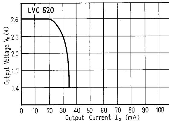
■LVC20 負荷特性/Load Charac.
