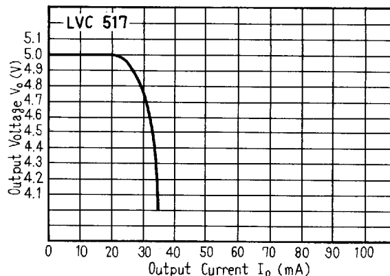
■ LVC517 負荷特性/Load Charac.
