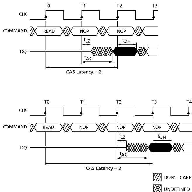
Figure 6 CAS Latency
