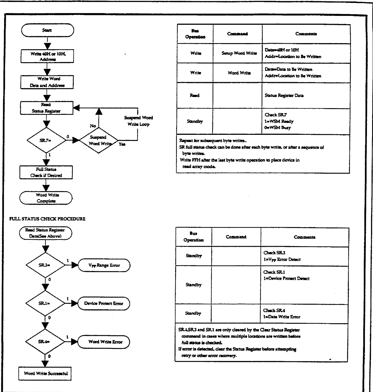
Figure5. Automated Word Write Flowchart
