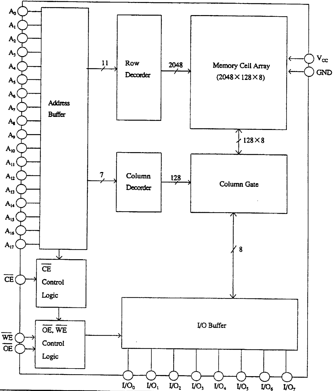
3. Block Diagram (V CC means S-V CC . A n means S-A n , where n=0 to 17.)
