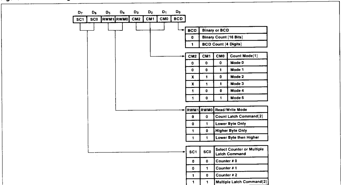
Figure 3. Control Register Format
