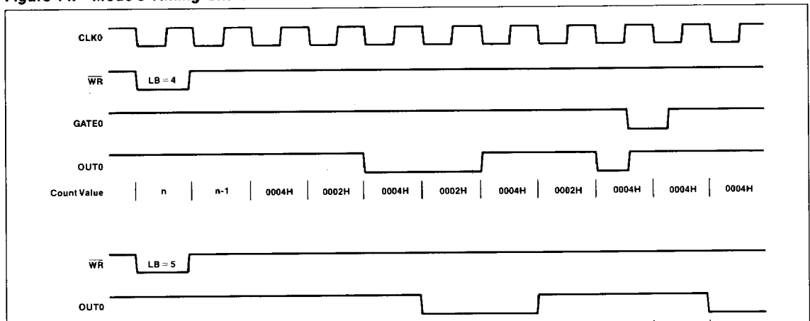
Figure 14. Mode 3 Timing Chart
