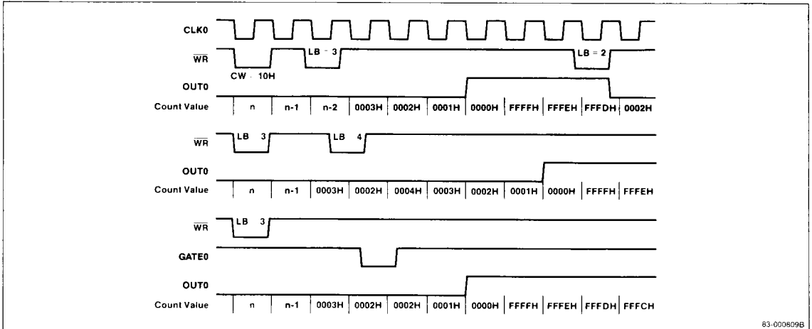
Figure 8. Mode 0 Timing Chart
