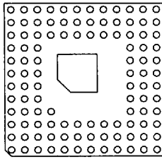
109 Pins 2 Without Window FP 03
