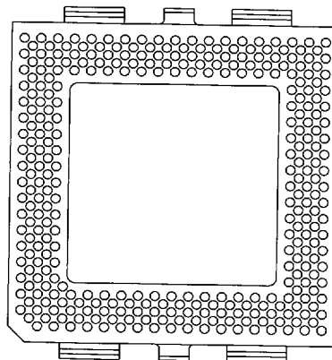
320 Pins B5* With Heatsink Tabs Intel Pentium™ P54CM
