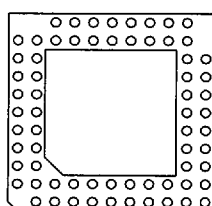
67 Pins 34 Without Window FP 35
