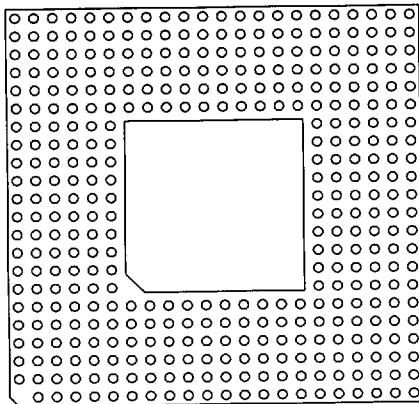
383 Pins 4 Without Window FP 03
