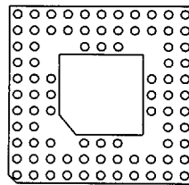
85 Pins 7 Without Window FP 8
