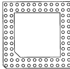
80 Pins 14 Without Window FP 15
