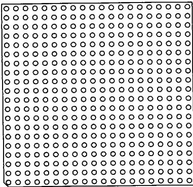
400 Pins 1
