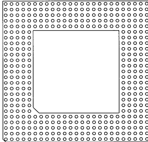
400 Pins 6
