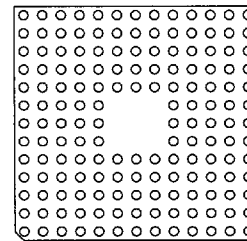
160 Pins 56
