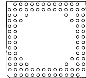
101 Pins 25
