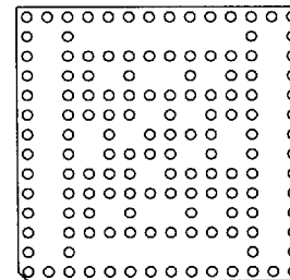
139 Pins 22
