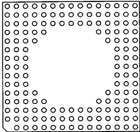
155 Pins 45
