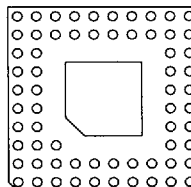
65 Pins 14
