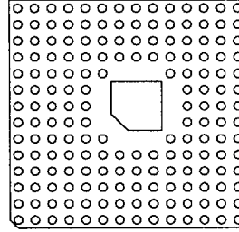
175 Pins 4
