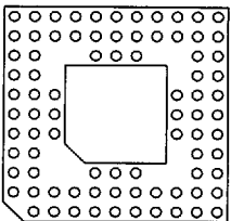
83 Pins 13 Without Window FP 14
