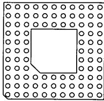
96 Pins 5 Without Window FP 6
