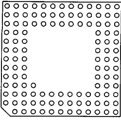
120 Pins 17
