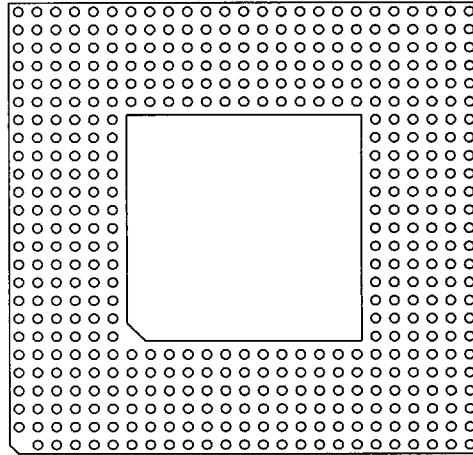
455 Pins 2
