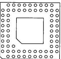
69 Pins 30 Without Window FP 31
