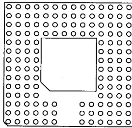
148 Pins 28
