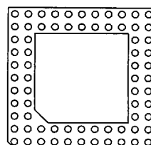
72 Pins 23 Without Window FP 24
