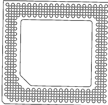
296 Pins A3 Without Window FP A2 Intel Pentium™ P54C
