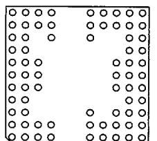
74 Pins 18
