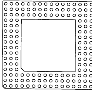
156 Pins 22 Without Window FP 24
