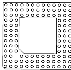
119 Pins 19 Without Window FP 20
