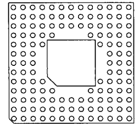
132 Pins 57
