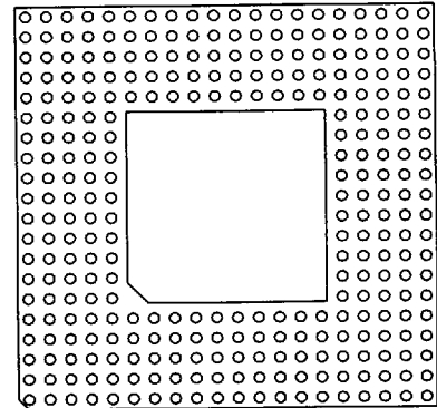
300 Pins 3 Without Window FP 09
