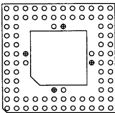
84 Pins 10 Without Window FP 11
