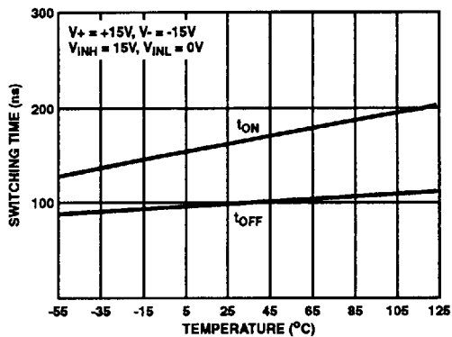
FIGURE 11. SWITCHING TIME vs TEMPERATURE, HI-304 THRU HI-307
