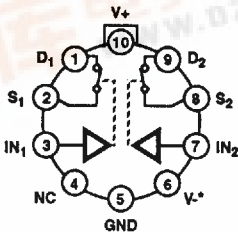
DUAL SPST HI-300 AND HI-304 TOP VIEWS
