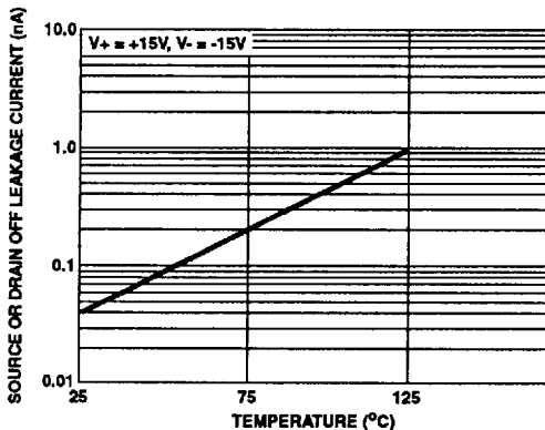
FIGURE 5. I_{S(OFF)} OR I_{D(OFF)} vs TEMPERATURE \uparrow
