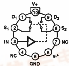
SPST HI-301 AND HI-305 TOP VIEWS
