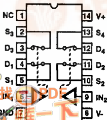
DUAL DPST HI-302 AND HI-306 (PDIP, CDIP, SOIC) TOP VIEW
