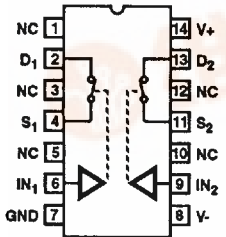
DUAL SPST HI-300 AND HI-304 TOP VIEWS
