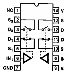
DUAL SPDT HI-303 AND HI-307 (PDIP, CDIP, SOIC) TOP VIEW
