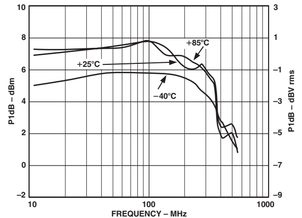
TPC 30. Output P_{1dB} vs. Frequency by Temperature, V_S = 5\text{ V} , R_L = 200\ \Omega , Maximum Gain
