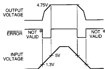
Figure 1. ERROR Output Timing
