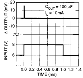
Line Transient
