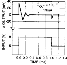
Line Transient
