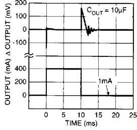
Load Transient
