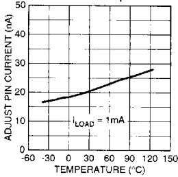
MIC29202/3 Adjust Pin Current vs. Temperature
