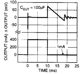
Load Transient
