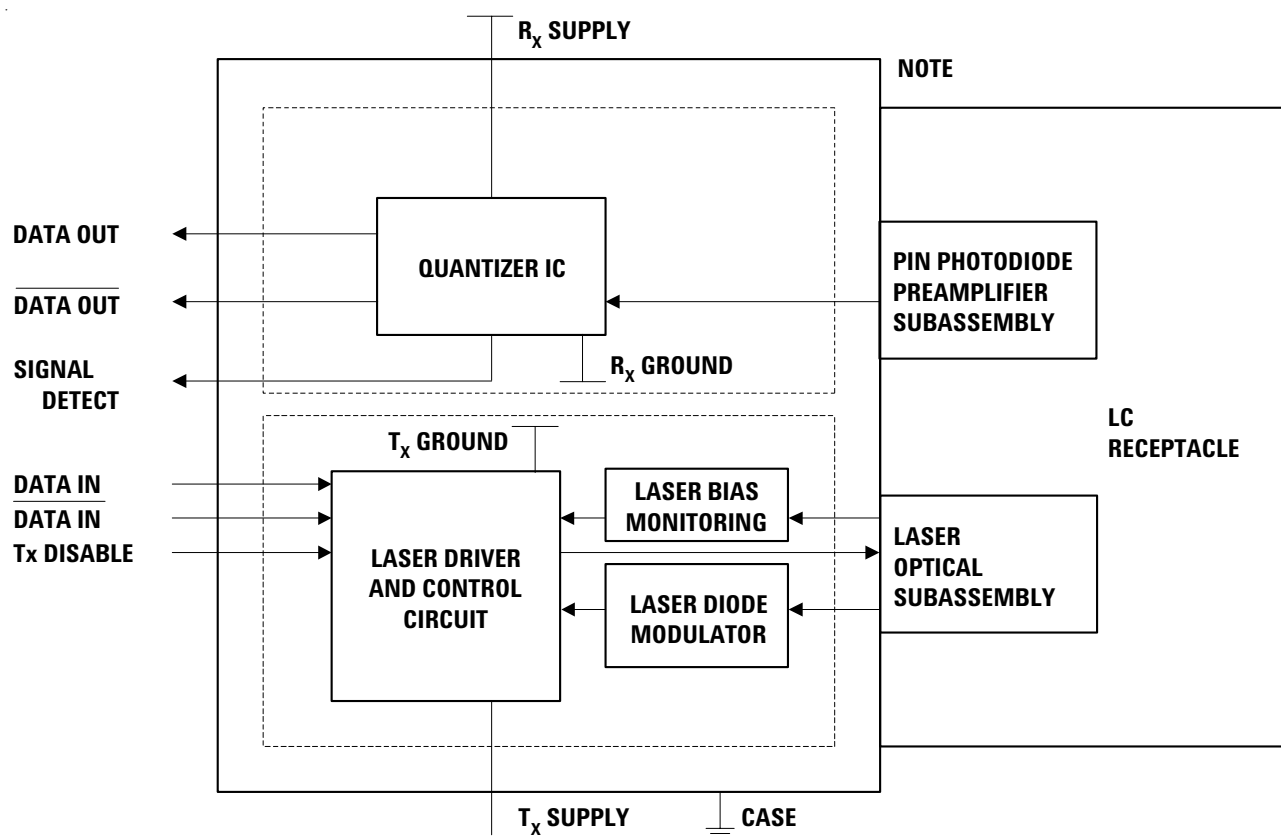
Figure 3. Block Diagram
