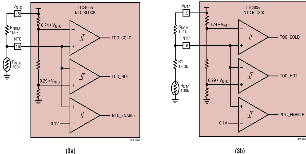
Figure 3. NTC Circuits
