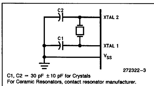
Figure 3. Oscillator Connections
