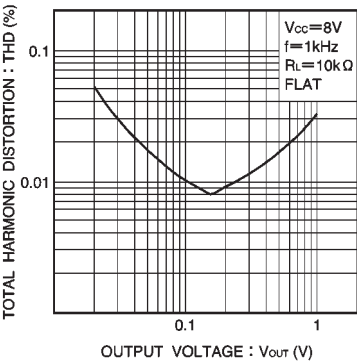
Fig. 8 Distortion vs. output voltage
