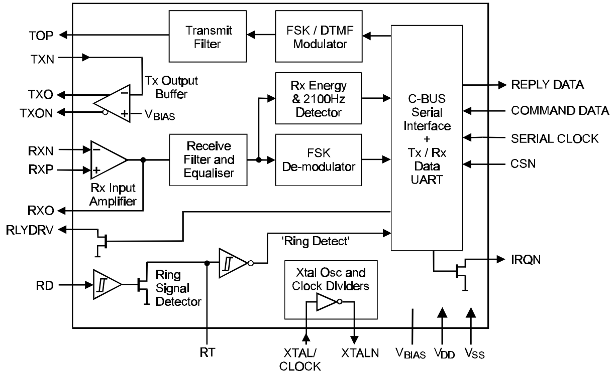
Figure 1 Block Diagram
