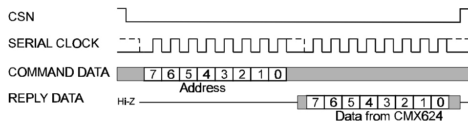
Figure 7 'C-BUS' Transactions
