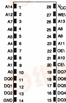
28-PIN ENCAPSULATED PACKAGE (720 Mil Extended)
